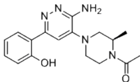
PC-4921001, DMSO-d 6
